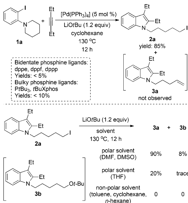
Scheme 2. Ligand effects on the carboiodination reaction and solvent effects on the stability of the product alkyliodide 2a .
